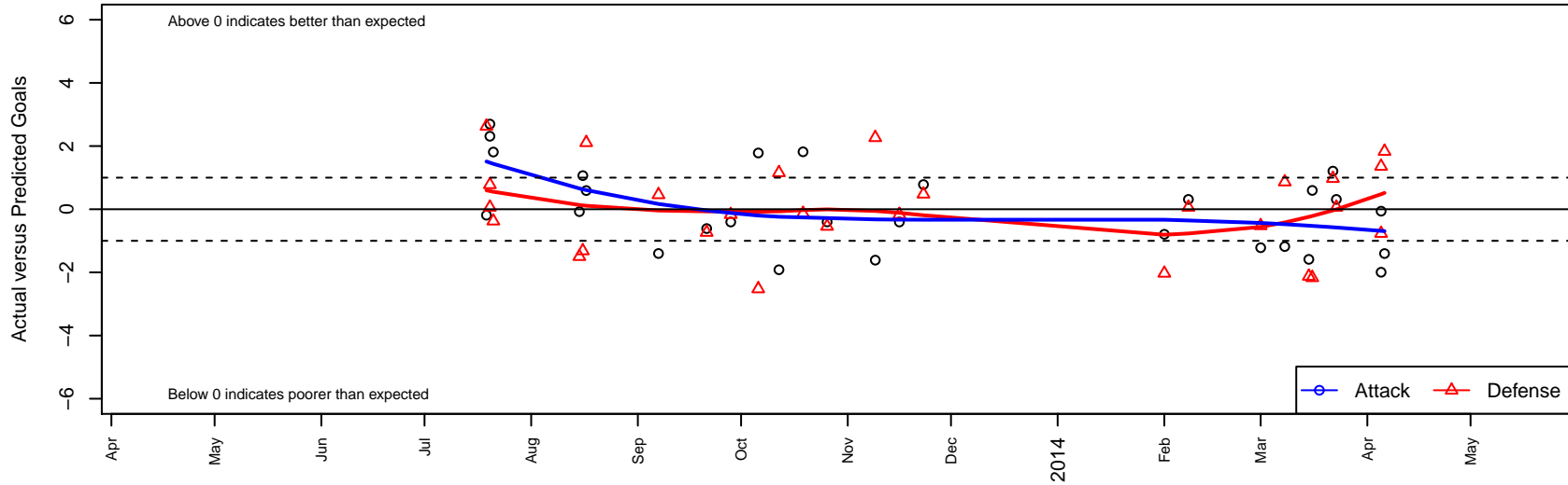
WPFC Fury Black B02 Dots are actual minus expected GF (blue circles) and GA (red triangles). Blue line is smoothed change in attack strength. Red is smoothed change in defense strength.
